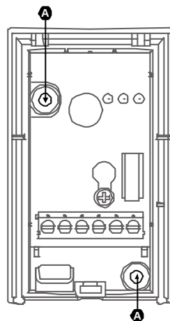
Fig. 2 - Detector Installation
