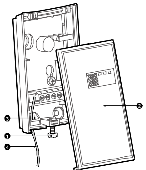
Fig. 3 - Detector Installation
